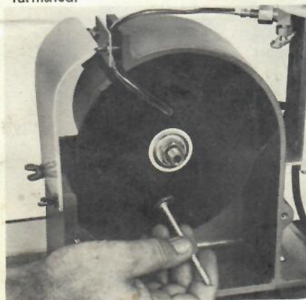
Sanding of gem stone with wet sanding paper. All necessary items furnished with Complete CAB-MATE.
