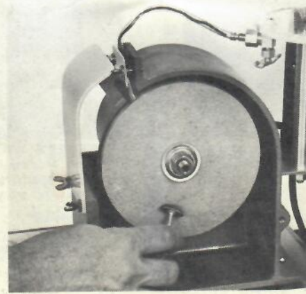
Final polishing of gem stone with felt pad. Sturdy 2-speed G.E. motor gives best polishing speed.
