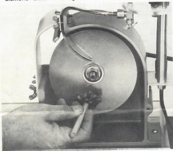
CAB-MATE handles all diamond tools; shown here with 6" diamond flat disc.
