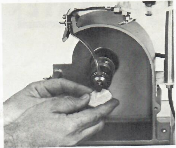
CAB-MATE with chuck for gemstone carving and jewelry work. Buffs jewelry too.
