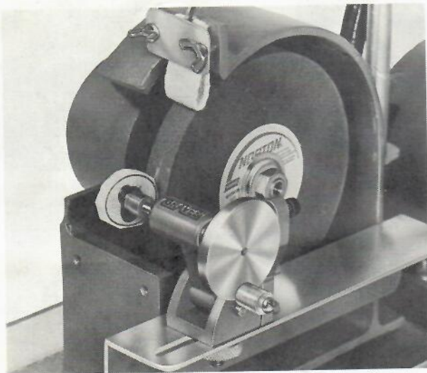
Here's where CAB-MATE does what others can't do! Preform Attachment makes accurate cabachon preforms in minutes. Follows template, every cab a "good" one. Attaches to any CAB-MATE in seconds.
